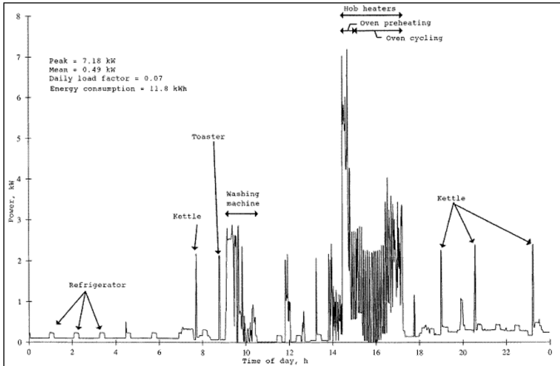
Figure I. Identification of Household Activities from Electricity Usage Data Unique Electric Load Signatures of Common Household Appliances
