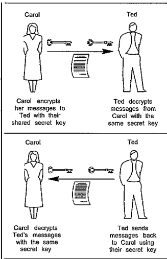
FIGURE 8-1. Secret-Key (Symmetric) Encryption
