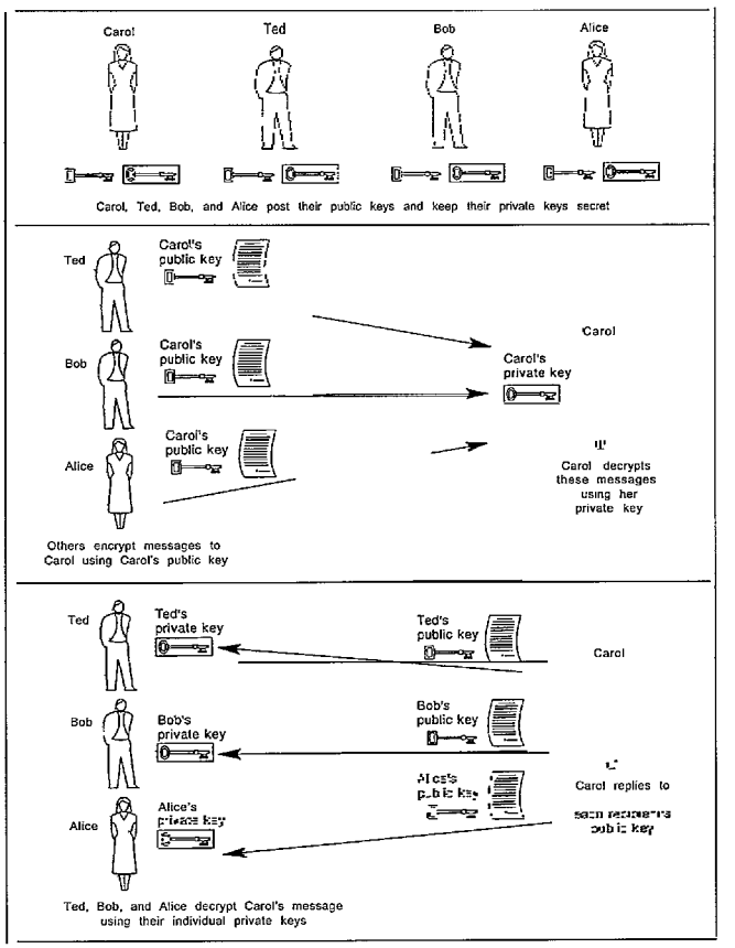
FIGURE 2-2: Public-Key Asymmetrical Encryption
