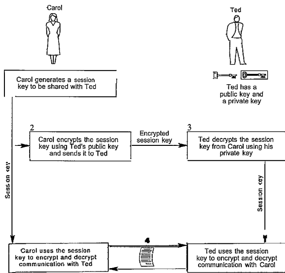
FIGURE 2-4: Secret-Key Distribution Using Public-Key Cryptography
