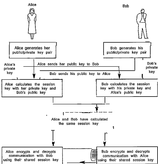
FIGURE 2-5: Diffie-Hellman Key Exchange
